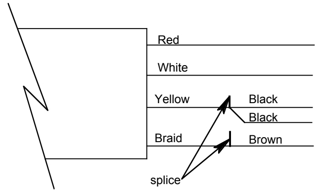
Splice Detail
