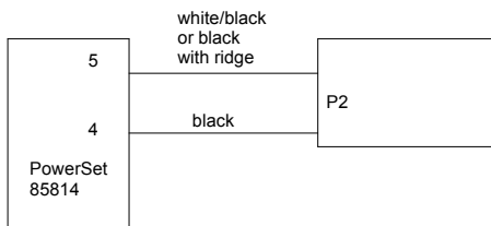
CONNECTION DIAGRAM
