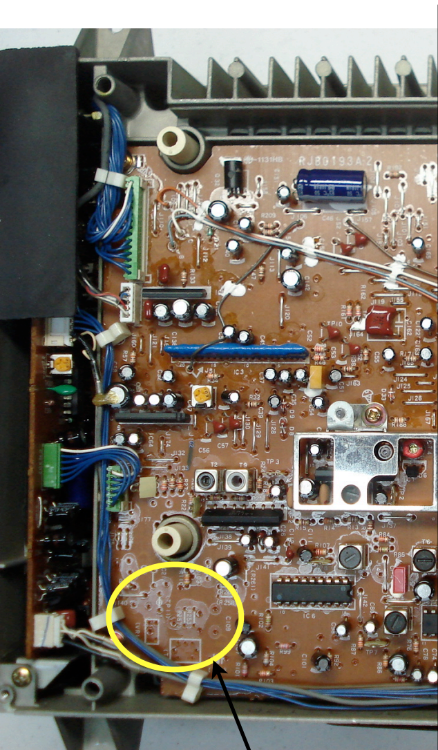
Area reserved for retrofit circuit board
